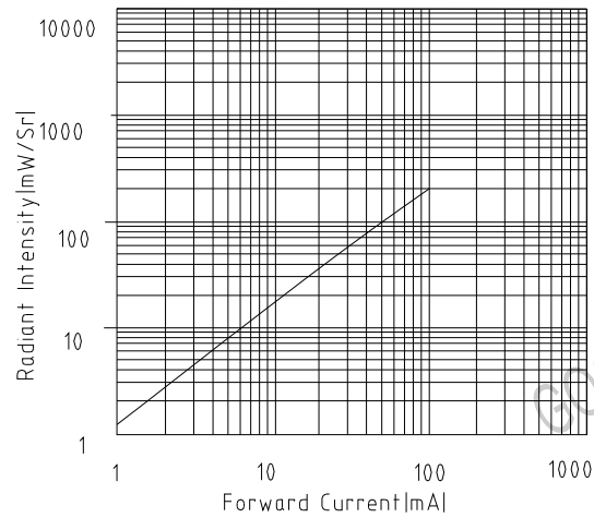
Fig.4 Forward Current Vs Radiant Intensity
