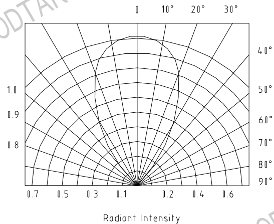
Fig.6 Angle Vs Radiant Intensity
