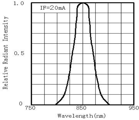
Fig.1 Spectral Distribution
