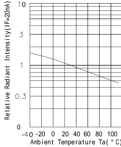
Fig.2 Relative Radiant Intensity Vs Ambient Temperature
