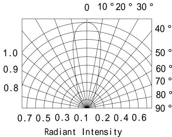
Fig.5 Angle Vs Radiant Intensity
